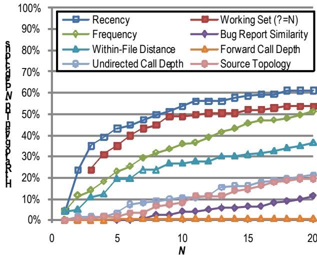
Figure 3. Model accuracy for click-based navigations, indicating the percentage of navigations that fell in the top- N predictions of each model. programmer to locations that he has previously visited. The two models were also able to accurately predict navigations in the Debug view because the participant used the debugger to repeatedly step over the same sections of code.
