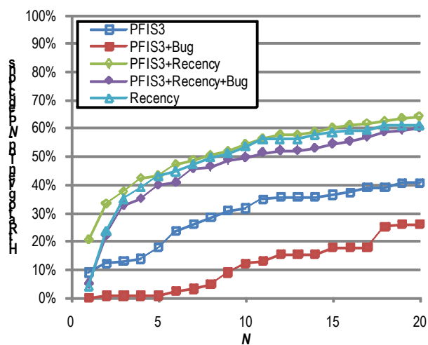
(a) Click-Based Navigations
