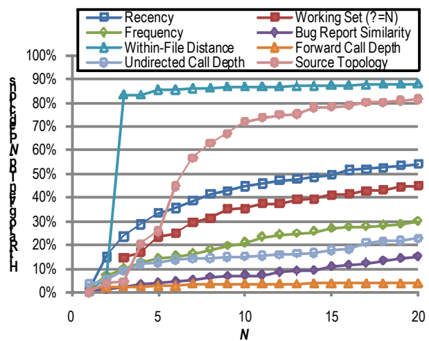
Figure 4. Model accuracy for view-based navigations.
